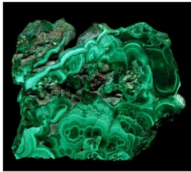
Malachite
