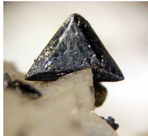
Tetrahedrite
