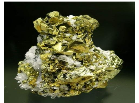
Chalcopyrite
