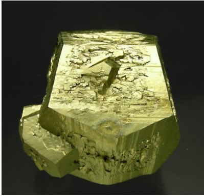
Pyrite
