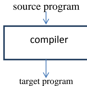
Figure 1.1 : A compiler
