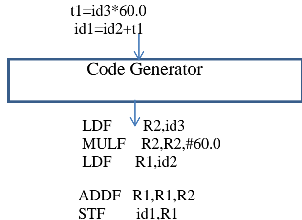
Fig 1.5: Translation of an assignment statement
