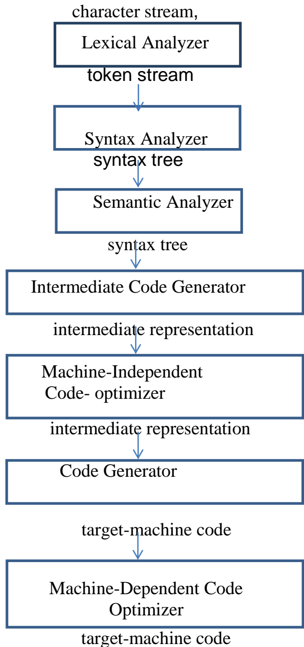
Figure 1.4: Phases of a compiler
