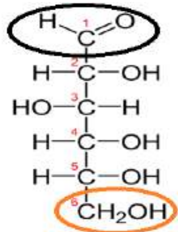
aldose glucose
