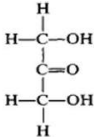
Dihydroxyacetone (ketose)
