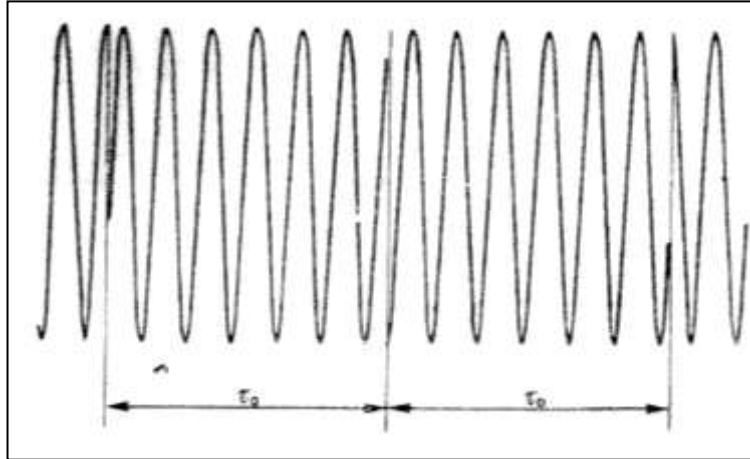
Fig. (2): Example of an e.m. wave with a coherence time of approximately \tau_c .
