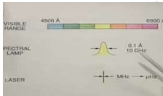
Figure (1): Comparison between the band width of lamp source and laser
