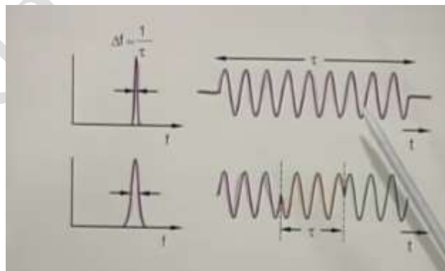
Figure (3): Coherence time between laser and lamp
