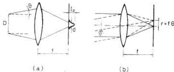
Fig (10): (a) Intensity distribution in the focal plane of a lens for a beam of divergence 0 (b) Plane-wave decomposition of the beam of a.
