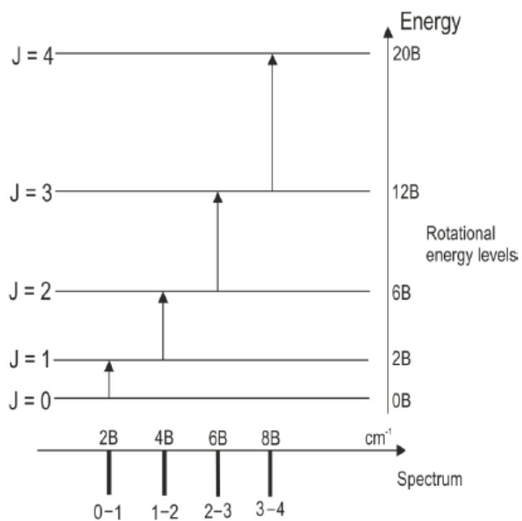
FIG. (18). Energy levels and spectrum of molecular rotation.
